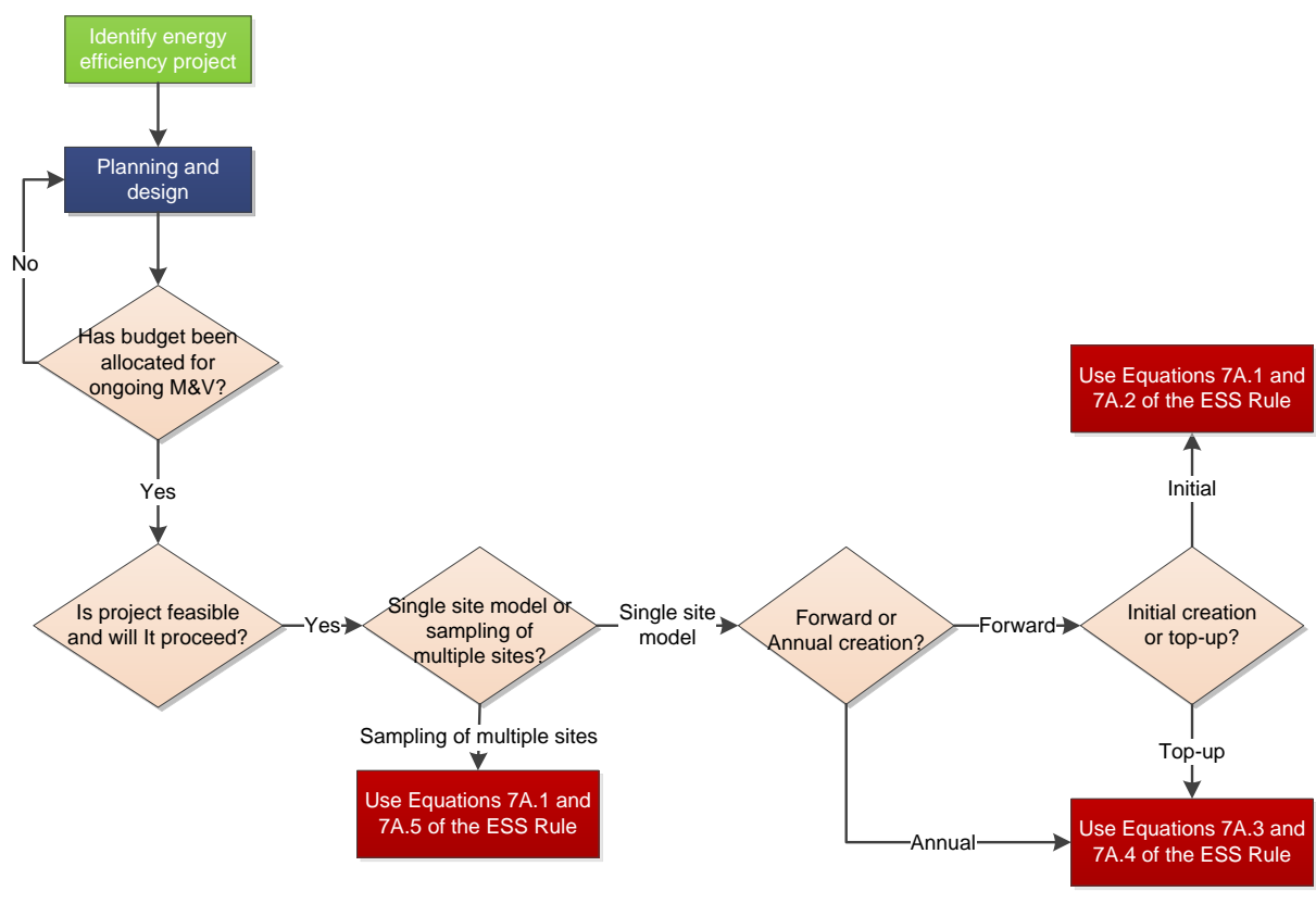
Figure 7.1 Determining which equation to use for calculating energy savings using the PIAM&V method
