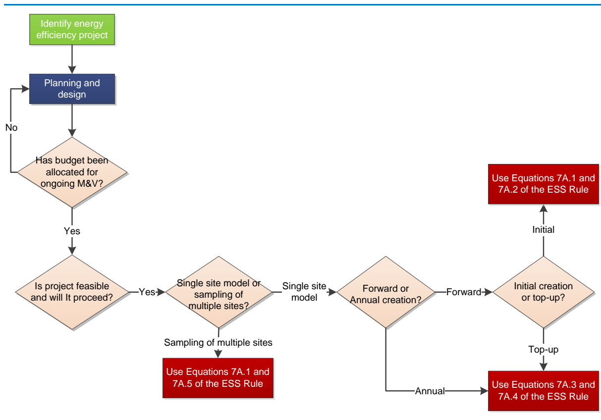
Figure 4.4.1 Determining which equation to use for calculating energy savings using the PIAM&V method
