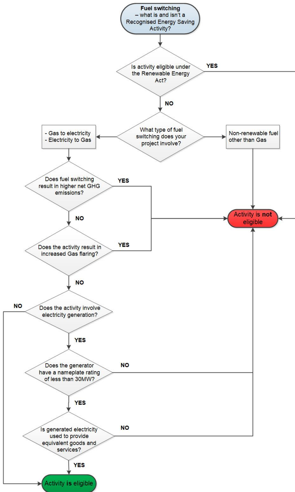
Figure D.1 Flowchart of eligible fuel-switching activities
